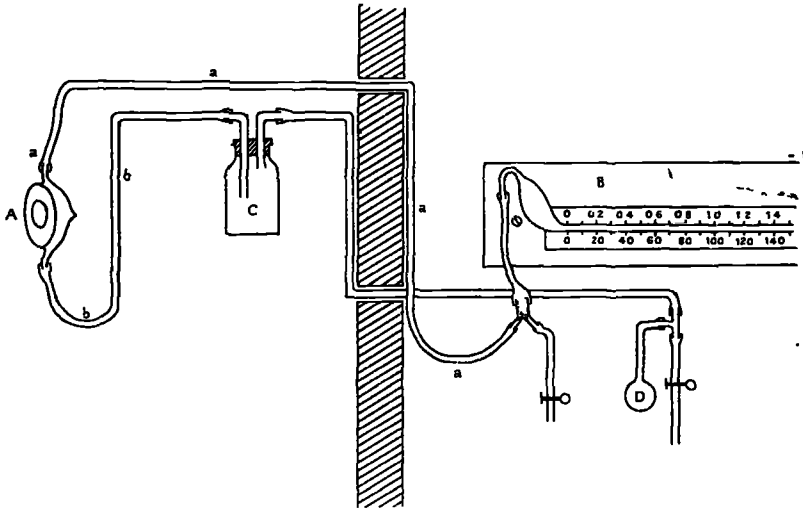
FIG. 1.—The apparatus used for recording the salivary secretion in experiments on conditioned reflexes. A , hemispherical bulb which is fixed over the fistula. aa , connecting tube leading through the partition separating the animal's room from the experimenter and connecting the bulb A to the registering apparatus, B . bb , tube connecting the bulb with bottle, C .
